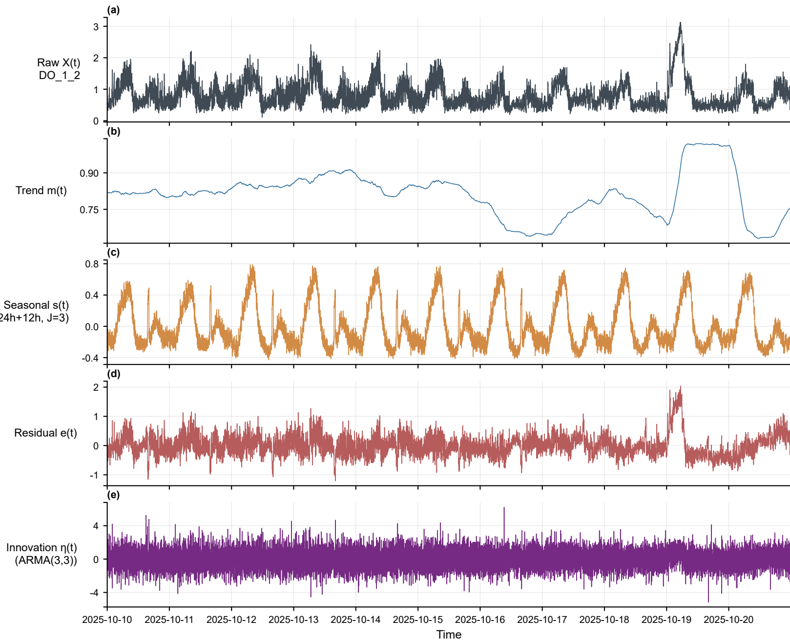
Multi-scale decomposition — DO_1_2 (aerobic, min) [2025-10-10~2025-10-20]
